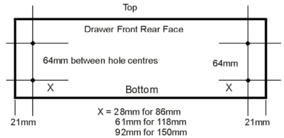
Bracket Positions (15mm carcass)
