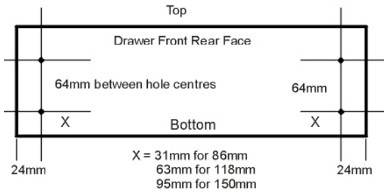
Bracket Positions (18mm carcass)
